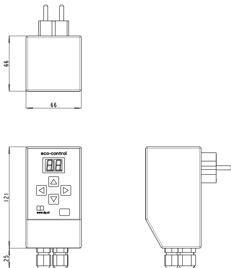
Figure 11: Dimensions ECO-Control
